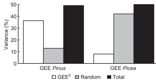
Fig. 6. Partition of variability contribution (%) of fixed effects and random effects for the GEE jack pine model ('GEE Pinus' in the x-axis) and GEE spruce model ('GEE Picea' in the x-axis) expressed as percentages of efficiencies (EF) of those covariates and total efficiencies shown in Table 5.
