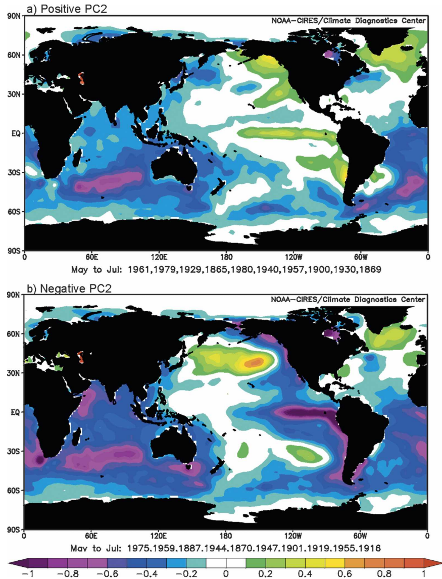
FIG. 8. May–July SST anomaly composites for 10 seasons of (a) highest PC2 scores and (b) lowest PC2 scores over the interval of 1854–1984. The anomalies were calculated from the mean of the reference period of 1971–2000. Years used in the composites are listed below each map.
