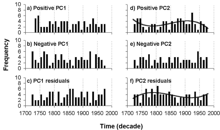
FIG. 9. Histograms showing the frequency per decade of PC1 and PC2 positive and negative departures exceeding the higher and lower 33.3% percentiles from the long-term mean of the reference period of 1718–1984. The frequency per decade of nondeparture years (PC residuals) is also shown. Third-order polynomial regression lines accounting for (d) 22.6% and (f) 20.4% are shown. PCs were obtained from the analysis of the BP, LN, and APe reconstructions.
