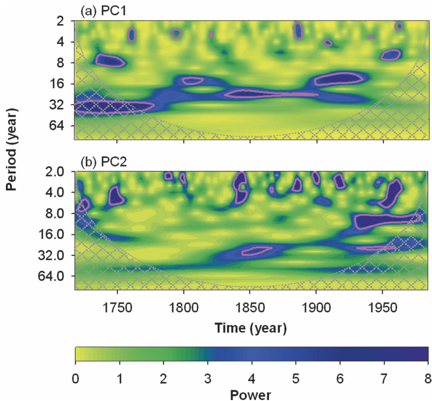
FIG. 6. Continuous wavelet transformation power spectra of (a) PC1 and (b) PC2. The dark blue color indicates areas of large power; thick-red contour is the 5% significance level for red noise [ AR(1) = 0.25 in (a) and AR(1) = 0.00 in (b)]. The cross-hatched regions on either end delineate the cone of influence where zero padding has reduced the variance. Note that for the period of 1718–67 the PCs were computed from only three climate reconstructions (BP, LN, and APe).
