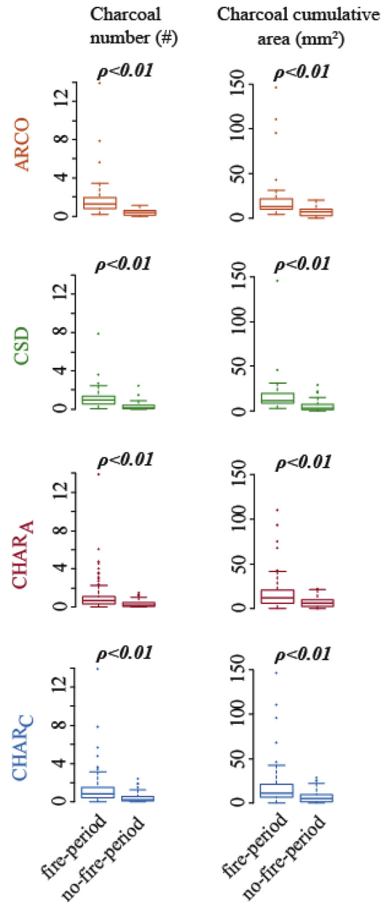
Fig. 4. Charcoal assemblages (number and area) of detected fire periods versus no-fire periods using CharAnalysis (CHARC in blue and CHARA in red), CSD (green) and ARCO (yellow). The p -values were obtained from Kolmogorov-Smirnov tests. (For interpretation of the references to color in this figure legend, the reader is referred to the Web version of this article.)
