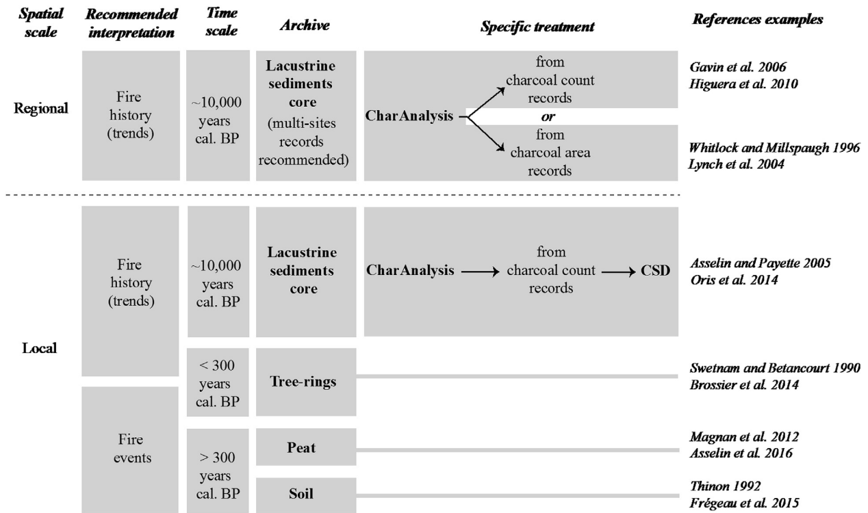
Fig. 6. Guidelines to select archive and proxy to reconstruct past fires in boreal forests.
