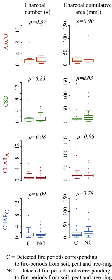
Fig. 5. Charcoal assemblages (number and area) of fire periods detected in lake sediments corresponding to fire periods detected or not in soil, peat and tree ring archives. Same color legend as in Fig. 4. The p -values were obtained from Kolmogorov-Smirnov tests. (For interpretation of the references to color in this figure legend, the reader is referred to the Web version of this article.)
