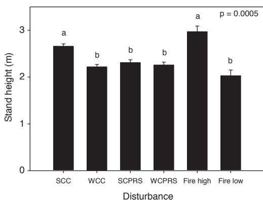
Fig. 4. Black spruce mean stand height ( m \pm 1 S.E) according to harvest treatment and soil burn severity. Values are adjusted means after controlling for time since disturbance. SCC=summer clearcut, WCC=winter clearcut, SCPRS=summer cut with protection of regeneration and soils, WCPRS=winter cut with protection of regeneration and soils; Fire high=high-severity soil burn; Fire low=low-severity soil burn. Disturbances identified by different letters are significantly different. Data for Fire high and Fire low from Simard et al. (2007).
