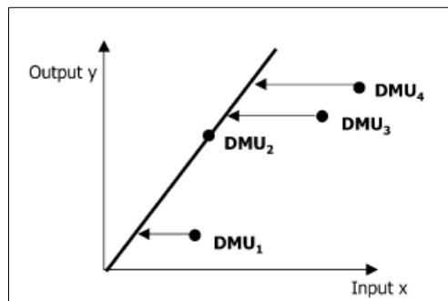
Figure 1.1 Data Envelopment Analysis (DEA) case of one input and one output presented by Homburg (2001).
