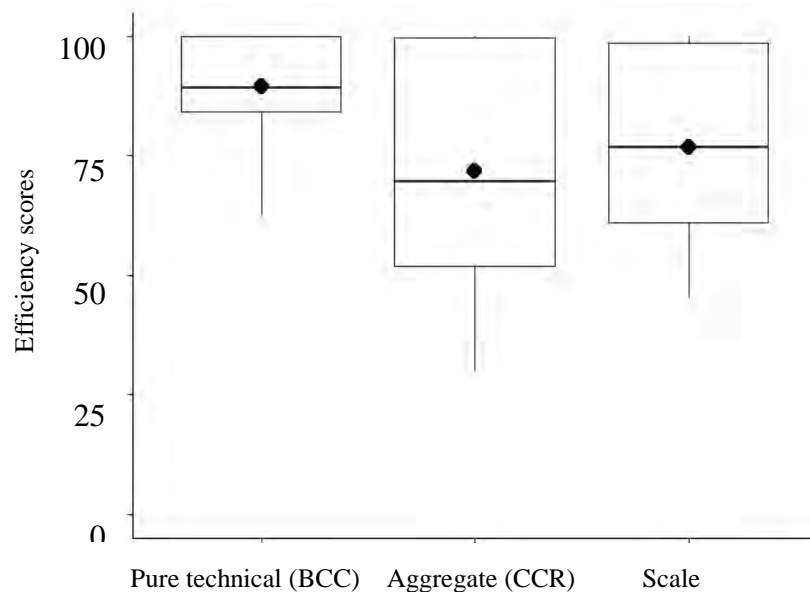
Figure 2.5 Efficiency scores of the DMUs that were examined. Black dots present the mean value. Boxplots follow the description detailed in Figure 2.2.
