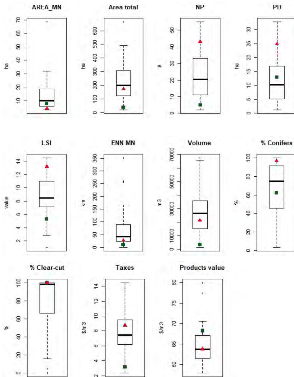
Figure 2.2 Box plots of variables for the 50 DMUs (for more details, see Table 2.1). The thick line represent the median (50 th percentile). The square represents the data among the 25th and 75th percentile presenting the 50% of data are located in this range. The extended lines are the variability outside the upper and lower percentiles. The points are extreme values. The example from figure 2.1 is presented as the red triangle showing the dispersed DMU (Figure 1a) and the green square the agglomerated DMU (Figure 1 b).
