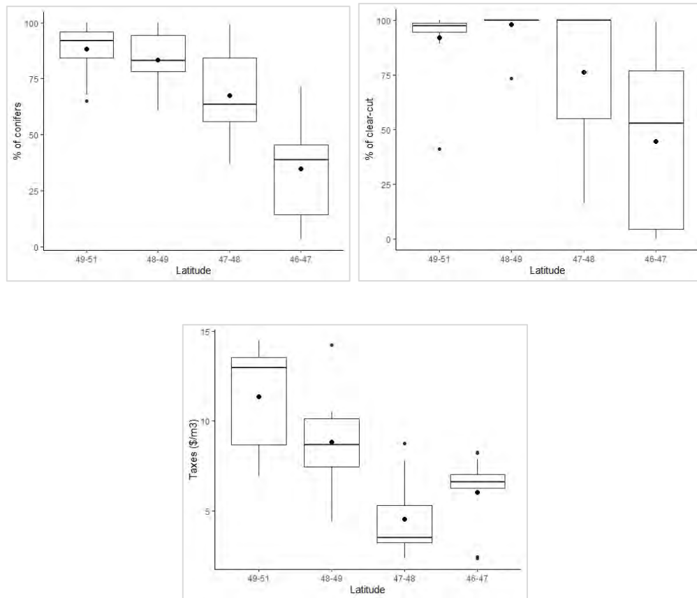
Figure 2.4. Boxplots of variables (% conifers, % clear-cut and taxes \$/m^3 ) used in the adjustment of the data envelopment analysis (DEA) by latitude. Dots present the mean value. Boxplots follow the description detailed in Figure 2.2.
