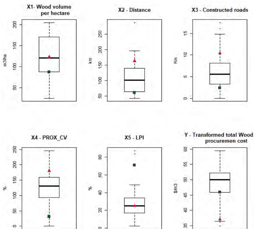
Figure 2.3 Boxplots of selected input variables: X1 = Wood volume per hectare (m 3 /ha), X2 = distance (km), X3 = constructed roads (km), X4 = PROX_CV (%), X5 = LPI (%), and output total wood procurement cost (Y) used in the data envelopment analysis (DEA). The points show the values from the DMU examples of dispersed DMU (Figure 1a), which are presented as red triangles and agglomerated DMUs (Figure 1b), which are as green squares. Boxplots follow the description detailed in Figure 2.2.
