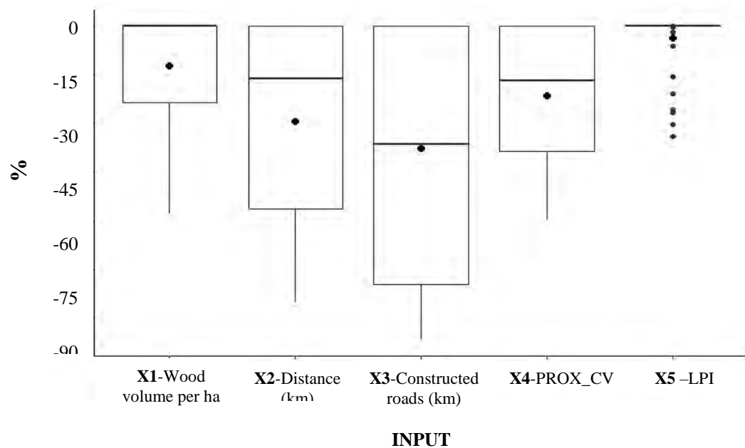
Figure 2.6 Target projections reductions for each input variable according to DEA analysis. Black dots present the mean value. Boxplots follow the description detailed in Figure 2.2.
