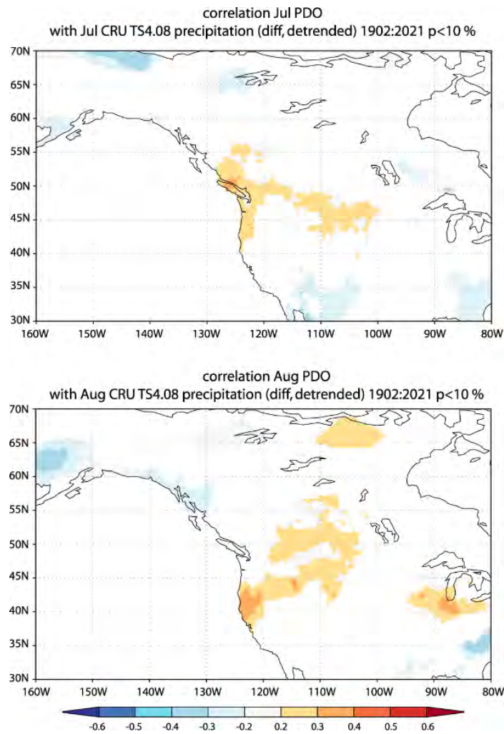
Figure S4.4 Correlation between July and August Pacific Decadal Oscillation (PDO) and CRU TS4.08 monthly precipitation fields over the 1902-2021 period. Colored areas indicate a significant level of correlation coefficient at p < 0.10 .
