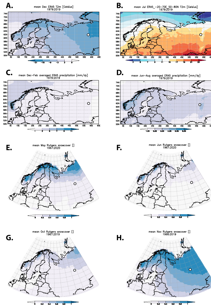
Figure S3.2 Climatology of the EBZ, based on the ERA5 reanalysis data. The snow cover data are available from https://doi.org/10.7289/V5N014G9 . A – mean December temperature, B – mean July temperature (both – in degree Celsius), C – mean winter (DJF) precipitation, D – mean summer precipitation (both – in mm/day). Snow cover depth, in m, for May (E), June (F), October (G) and November (H). The empty circle represents the study area.
