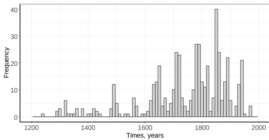
Figure S4.6 Frequency of tree pith dates for sampled dead and live trees over time.
