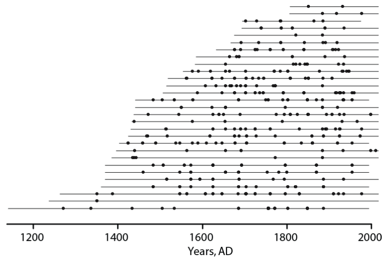
Figure 3.2 Dendrochronological reconstruction of the fire history in the Pechora-Ilych BR over the 1271–2010 period. A single straight line represents each study site, and a dark circle represents a fire event.
