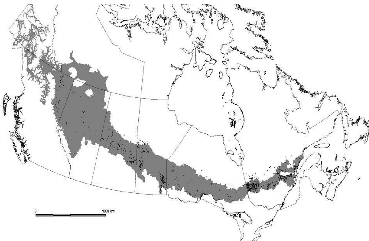
Figure 1.1 Map of the study area, along an east-west transect in Canada. The light grey area represents the “boreal mixedwood” ecoregion of Canada (Source: Baldwin et al. 2012). Black spots represent our study sites.
