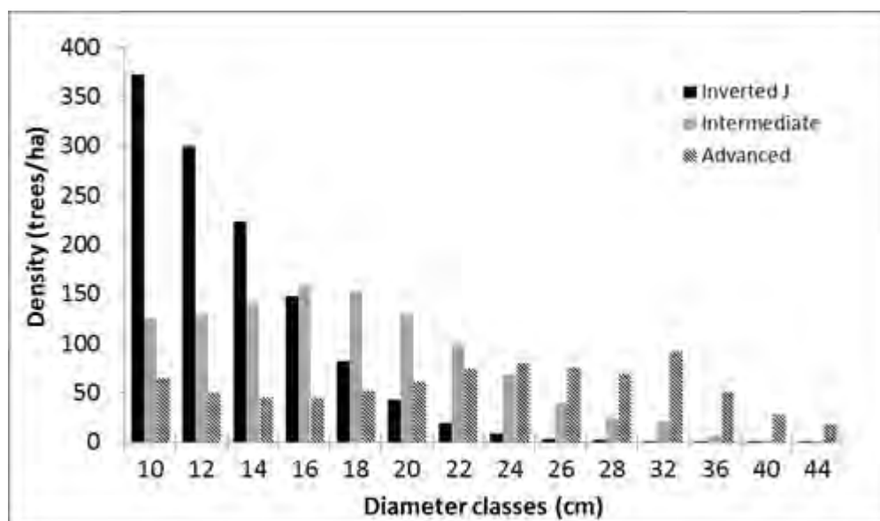
Figure 2.2 Mean diameter distributions corresponding to the three types of stand structure. Black bars represent the "inverted J" structure, gray bars represent the "intermediate" structure and hatched bars indicate the "advanced" structure.
