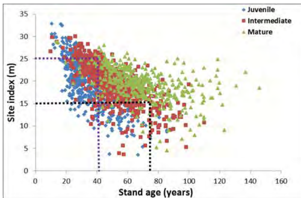
Figure 2.3 Distribution of structural types based on the site productivity and stand age. 1688 aspen stands were used in analysis; including 603 "inverted J" (diamond), 650 "intermediate" (square) and 435 "advanced" (triangle) structure.
